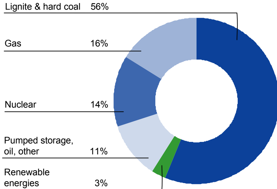
Fuel mix 2007 (capacity in %) Total generation capacity 2007: 45 GW
