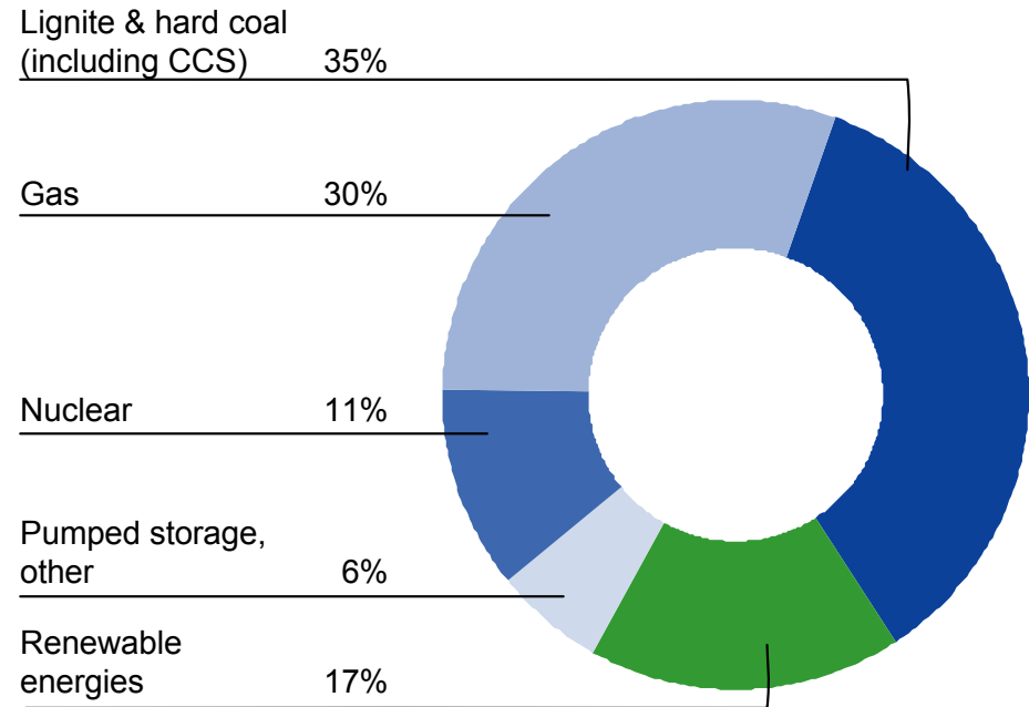
Vision fuel mix 2020 (capacity in %)*) Total generation capacity 2020e: ca. 60 - 70 GW
