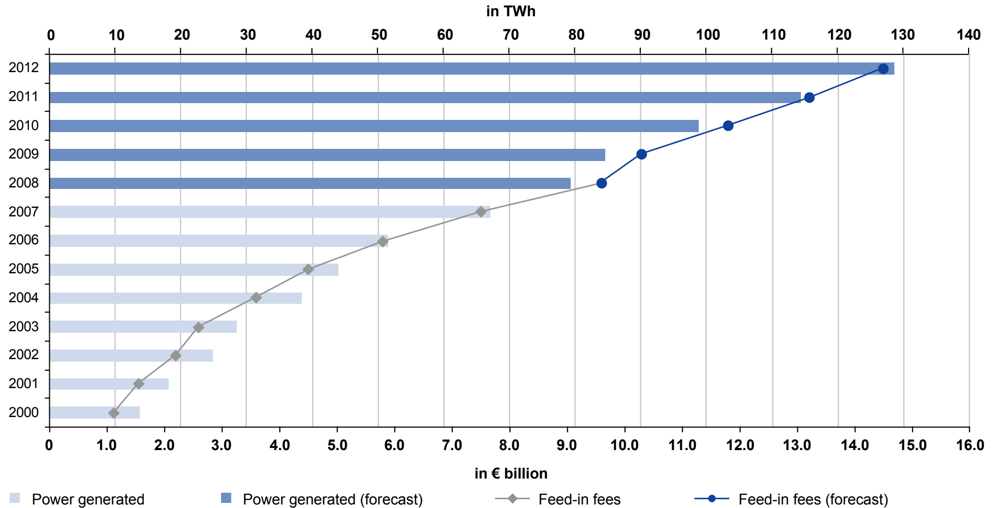
Development of power generated in accordance with the German Renewable Energy Act (REA) and REA surcharges for 2000 – 2012 (forecast)
